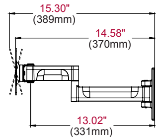
SIDE VIEW EXTENDED +/-15° TILT
